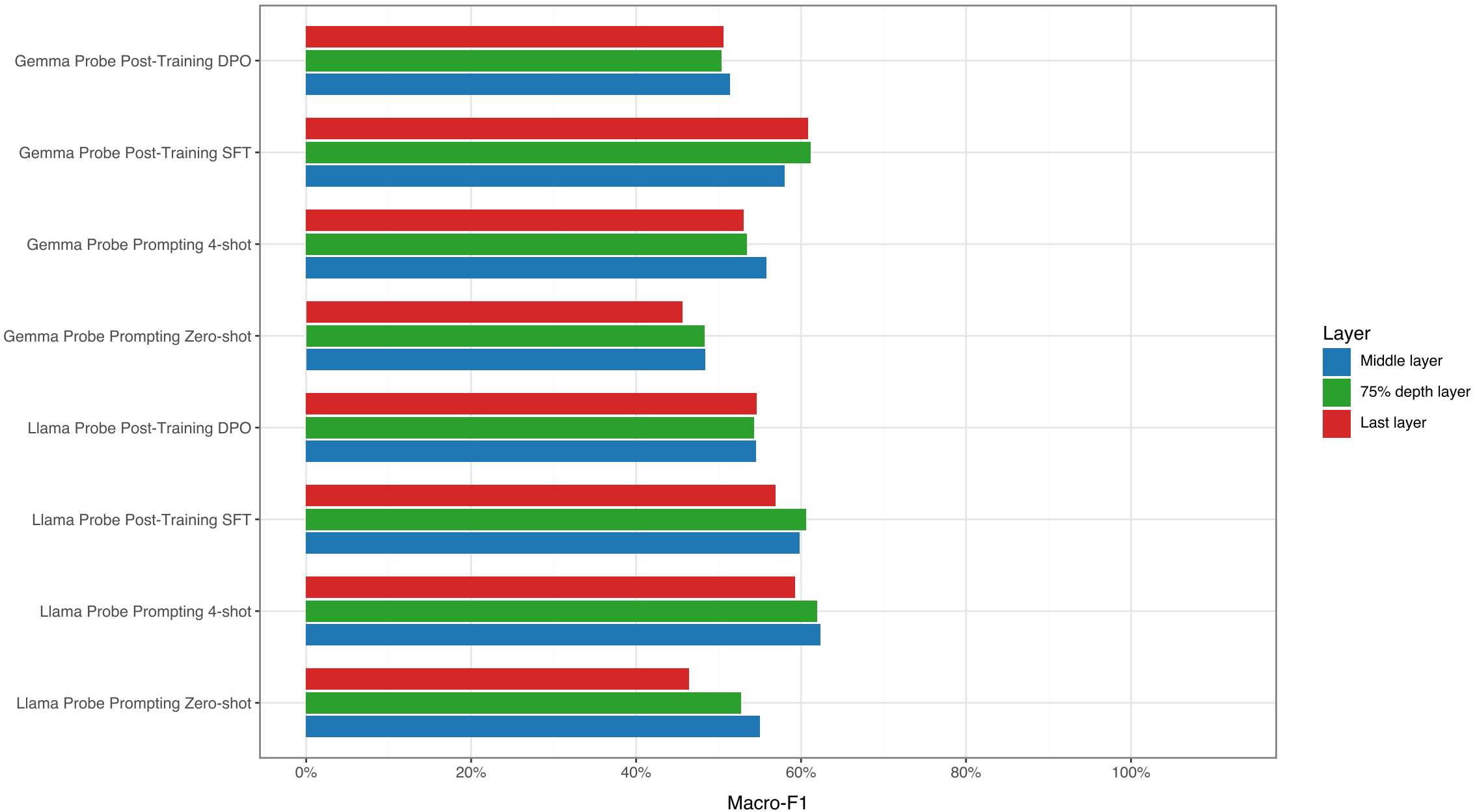
Probe Layer Macro-F1 on When2Call
